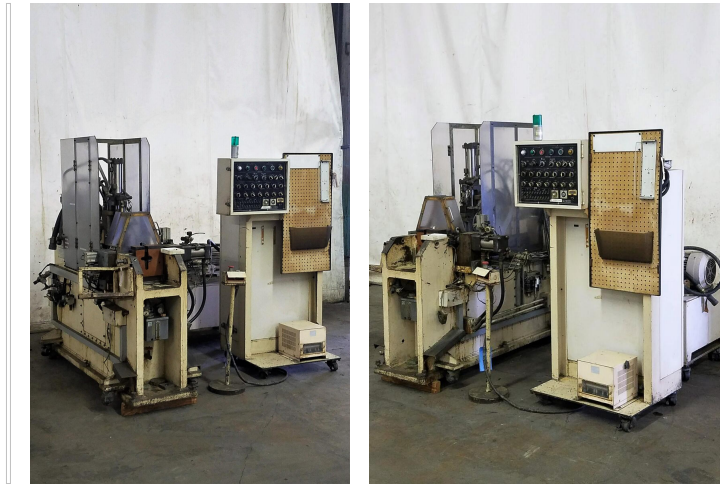
Taisei PHD-254DT Tube End Former with Secondary Clamps
