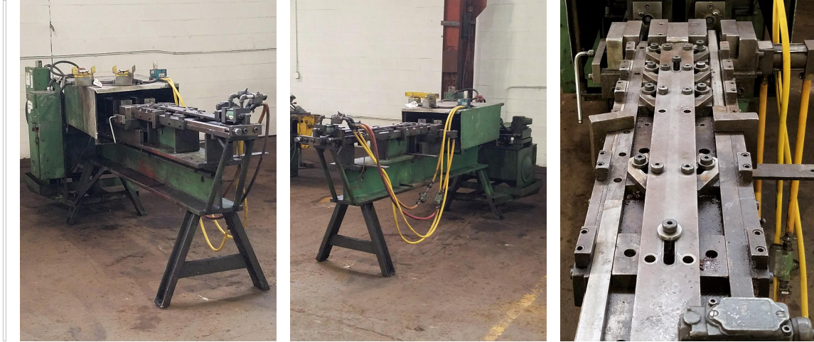
2" Hydraulic Swager Tube End Finisher
